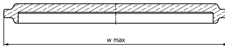
FIG. X2.2 Deviation from Flatness
