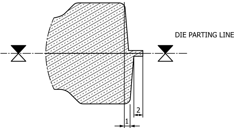
FIG. X2.4 Flash Projection
