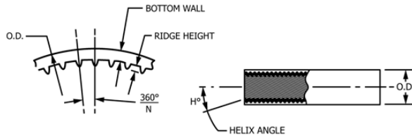
FIG. 3 Inside Diameter Enhanced Tube Nomenclature
